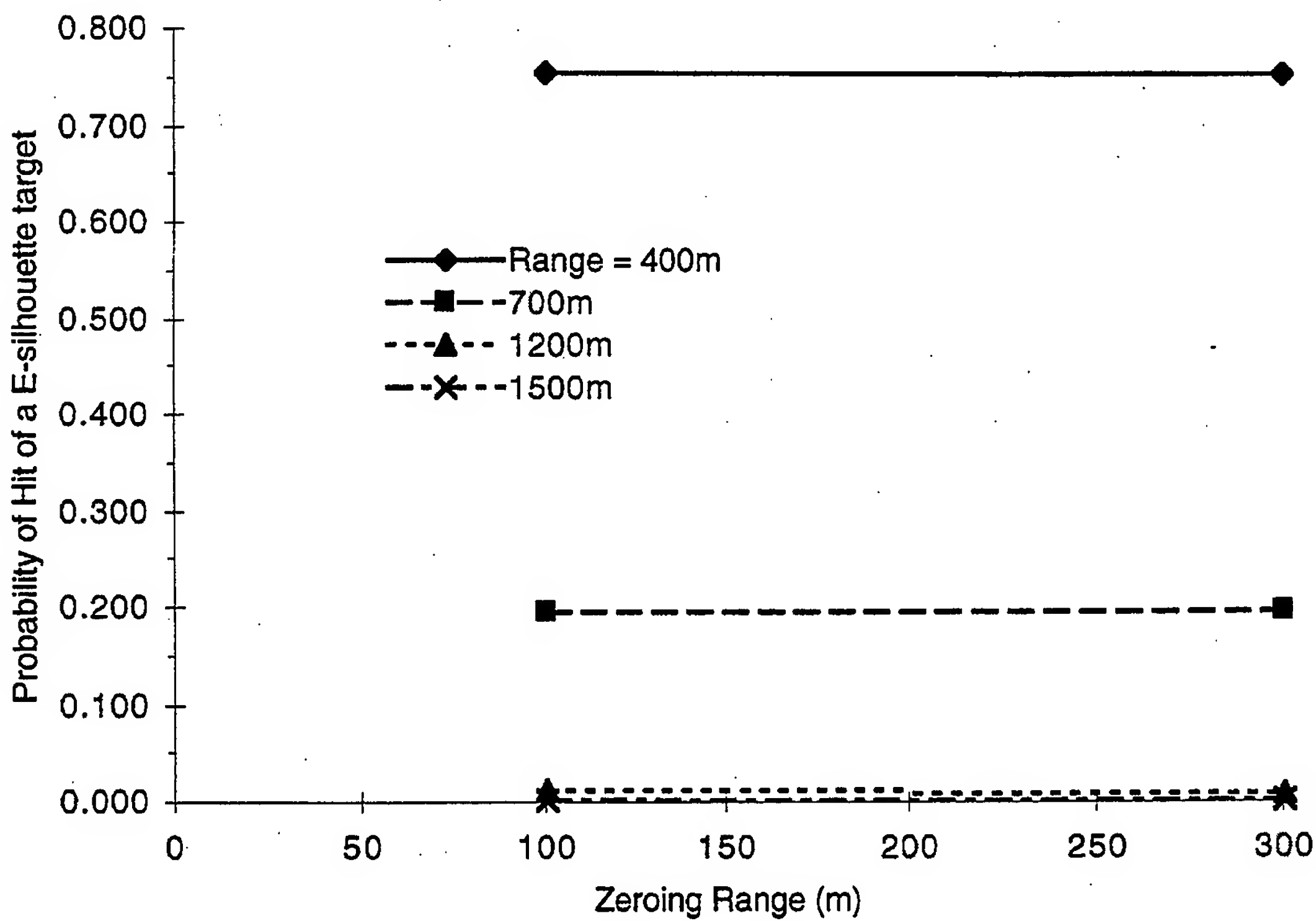
Figure D-3. Error Budget Sensitivity Zeroing Range.
